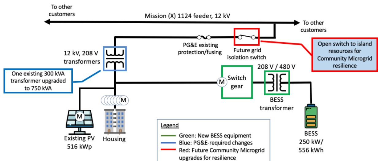
Valencia Gardens Apartments with existing solar
